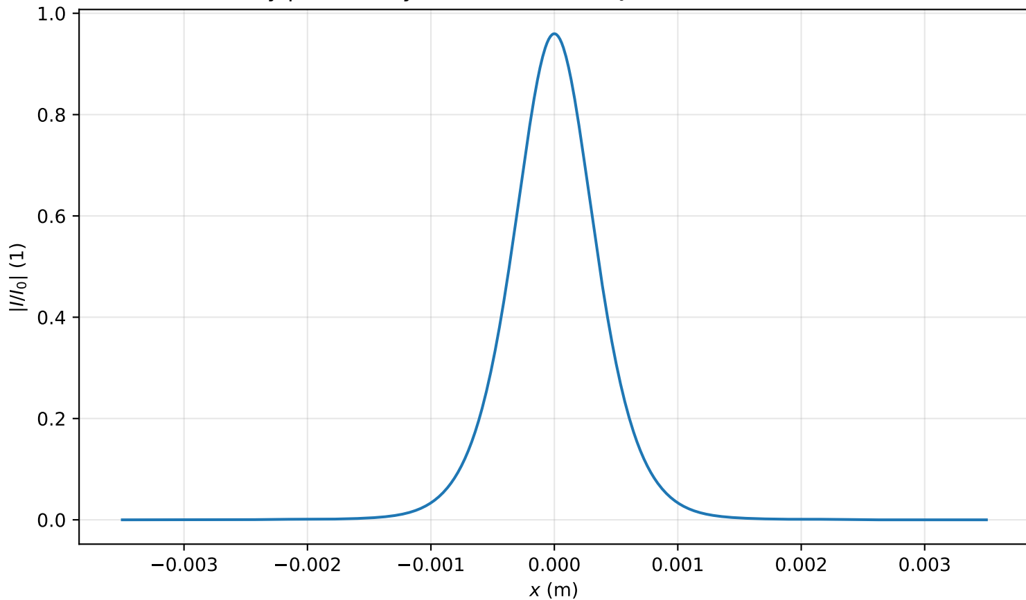
Intensity profile I(x, y = 0, z = 3.582m)/I_0 , P_{in}=0.8P_{cr} , artificial time
